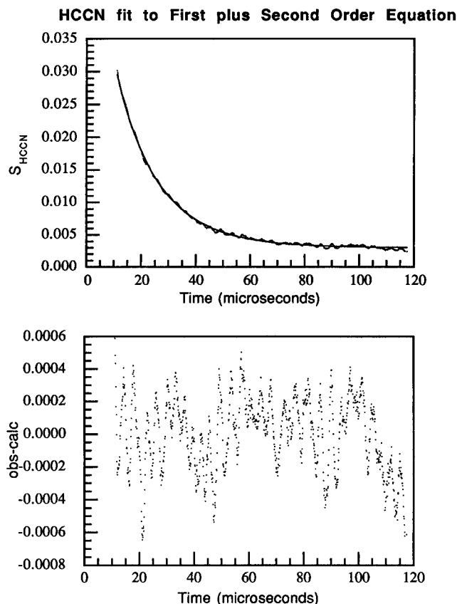
Figure 2. Typical fit of HCCN with first plus second-order equation (eq 5); with 50 mTorr of NO and total pressure of 6.2 Torr; residuals are shown below the plot. The ordinate scale is in base e absorbance units.
