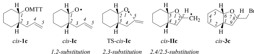
Fig. 3 Convention used in this article for numbering atoms in product classes associated with alkoxyl radical reactions, exemplified for alkenoxythiazolethione cis-1c , derived 4-alkenoxyl radical cis-1c , the transition structure for the 5-exo-cyclization TS-cis-1c , 5-exo-cyclized carbon radical cis-1lc , and bicyclic bromocyclization product cis-3c .
