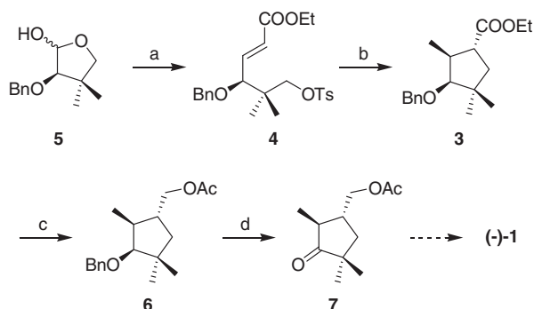
Scheme 2. Reagents and conditions: (a) (i) \text{Ph}_3\text{P}=\text{CHCOOEt} , toluene, reflux, 8 h, 75%; (ii) \text{TsCl} , py, DMAP, rt, 24 h, 88%; (b) \text{Me}_2\text{CuLi} , \text{TMSCl} , -78^\circ\text{C} to rt, THF, 24 h, 94%; (c) (i) \text{LiAlH}_4 , THF, 0^\circ\text{C} , 0.5 h, 95%; (ii) \text{Ac}_2\text{O} , DMAP, py, DCM, rt, 92%; (d) (i) 10% \text{Pd/C} , \text{H}_2 , MeOH, 24 h, 96%; (ii) Dess–Martin periodinane, DCM, 0^\circ\text{C} , 1 h, 93%.
