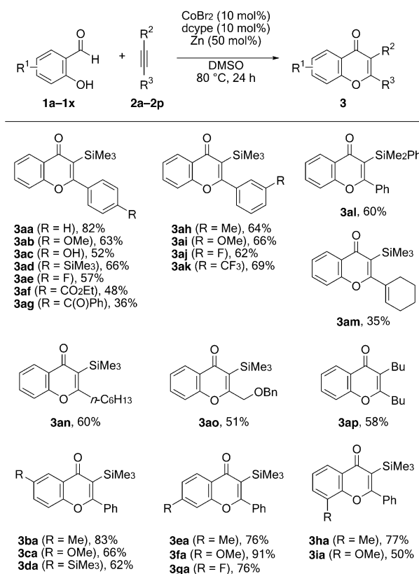
Scheme 2. Scope of the dehydrogenative annulation reaction of salicylaldehydes with silylacetylenes and dialkylacetylenes (0.3 mmol scale).
