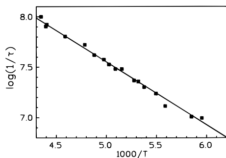
Figure 1. Arrhenius plot for 1,2-H shift in \text{C}_6\text{H}_5(\text{CH}_3)\text{CH}-\ddot{\text{C}}-\text{Cl} obtained by measuring the rate of decay of carbene in isooctane at 305 nm.
