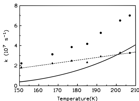
Figure 4. Quenching of \text{C}_6\text{H}_5(\text{CH}_3)\text{CH}-\ddot{\text{C}}-\text{Cl} by TME in methylcyclohexane as a function of temperature: ●, k_{\text{obs}} = k_1 + k_q[\text{TME}] . Solid line calculated from A and E_a in methylcyclohexane: ▲, k_q[\text{TME}] with [TME] = 0.4 M.
