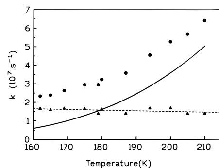
Figure 3. Quenching of \text{C}_6\text{H}_5(\text{CH}_3)\text{CH}-\ddot{\text{C}}-\text{Cl} by TME in isooctane as a function of temperature: ●, k_{\text{obs}} = k_1 + k_q[\text{TME}] . Solid line calculated from A and E_a in isooctane: ▲, k_q[\text{TME}] with [TME] = 0.21 M.
