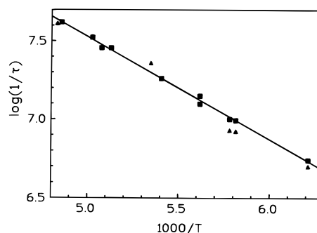
Figure 2. Arrhenius plot for \text{C}_6\text{H}_5(\text{CH}_3)\text{CH}-\ddot{\text{C}}-\text{Cl} in decalin at 305 nm: ■, no TME; ▲, [TME] = 1.0 M.
