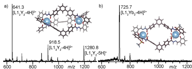
Figure 3. Mass spectra and minimized structures (SPARTAN, AM1 force field) of (a) [\text{I}_3\text{Y}_2]^{6-} and (b) [\text{I}_2\text{Yb}_2]^{2-} .
