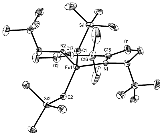
Figure 6. Molecular structure of (S)-('BuBox)Fe(CH 2 SiMe 3 ) 2 ( 11 ) with 30% probability ellipsoids. Hydrogen atoms omitted for clarity.
