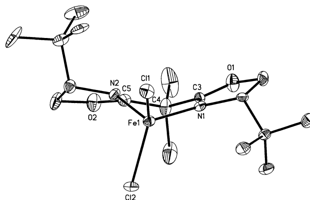
Figure 1. Molecular structure of (S)-('BuBox)FeCl 2 ( 3 ) with 30% probability ellipsoids. Hydrogen atoms omitted for clarity.
