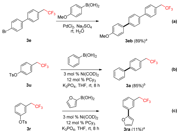
Scheme 3. Further Functionalization of Some Products
