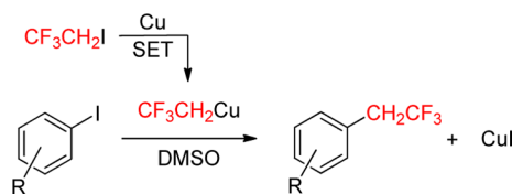
Scheme 4. Proposed Mechanism
