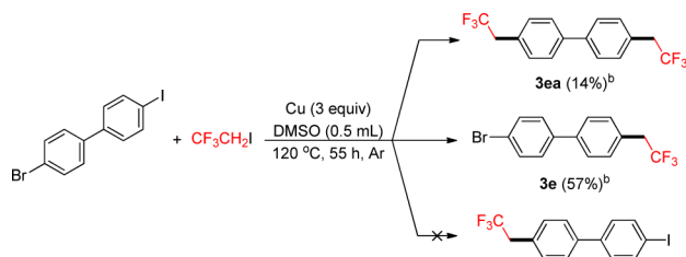
Scheme 2. Site-Selective Reductive Coupling a
