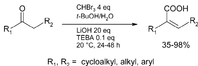
Scheme 1. One-pot reaction of ketones with bromoform. 22
