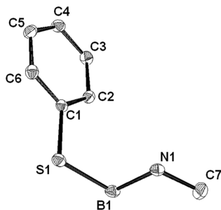
Figure 6. Molecular structure of 19 , with thermal ellipsoids at the 50% probability level. All hydrogen atoms omitted for clarity.
