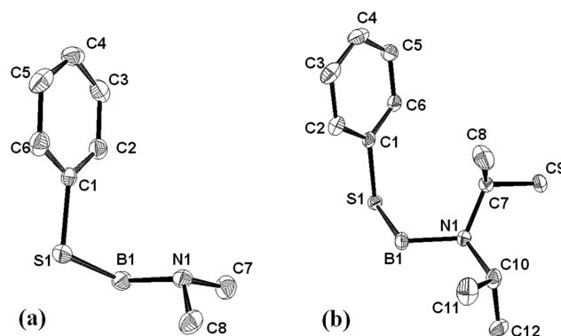
Figure 3. Molecular structures of amine-thioboranes (a) 11a and (b) 11b, with thermal ellipsoids at the 50% probability level. All hydrogen atoms omitted for clarity.
