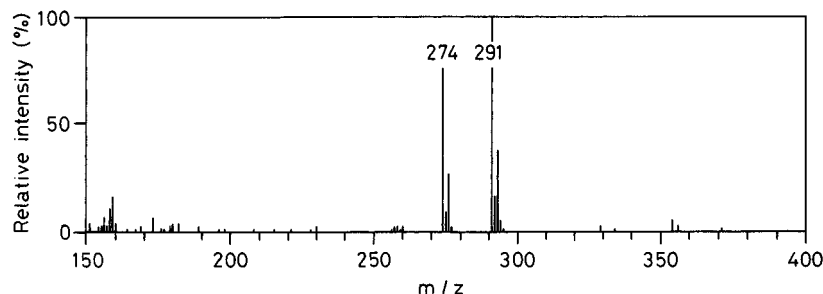
Figure 2. Thermospray liquid chromatography mass spectrum of a chlorination byproduct of thiobencarb.
