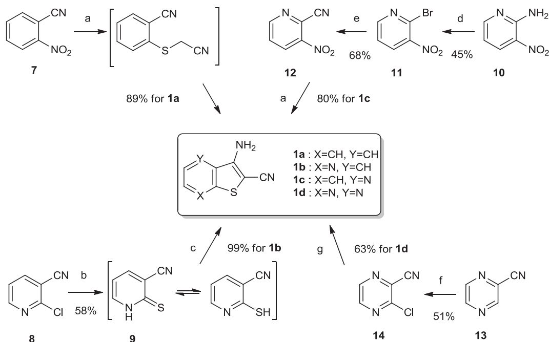
Scheme 2. Reagents and conditions: a) \text{HSCH}_2\text{CH}_2\text{CN} , \text{KOH}/\text{DMF} , 0^\circ\text{C} , 15 min then \text{BrCH}_2\text{CN} , 0^\circ\text{C} , 2 h; b) thiourea, ethanol, 120^\circ\text{C} ( \mu\text{W} ), 45 min; c) \text{ClCH}_2\text{CN} , \text{K}_2\text{CO}_3 , acetone, r.t., 4 h; d) \text{KNO}_2 , \text{CuBr} , \text{HBr} 48%, \text{DMSO} , 35^\circ\text{C} , 4 h; e) \text{CuCN} , fusion 150^\circ\text{C} , 2 h; f) \text{SO}_2\text{Cl}_2 , toluene- \text{DMF} , r.t., 5 h; g) \text{NaHS} , r.t., 3 h then \text{BrCH}_2\text{CN} , \text{K}_2\text{CO}_3 , acetone, r.t., 3 h.
