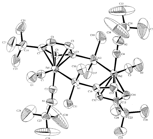
Figure 4. ORTEP drawing of 13c .
