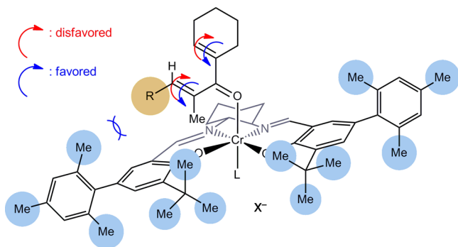
Scheme 4. Proposed Model to Rationalize Enantioselectivity
