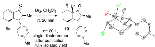
Scheme 3. Absolute Stereochemistry of Nazarov Product 9e
