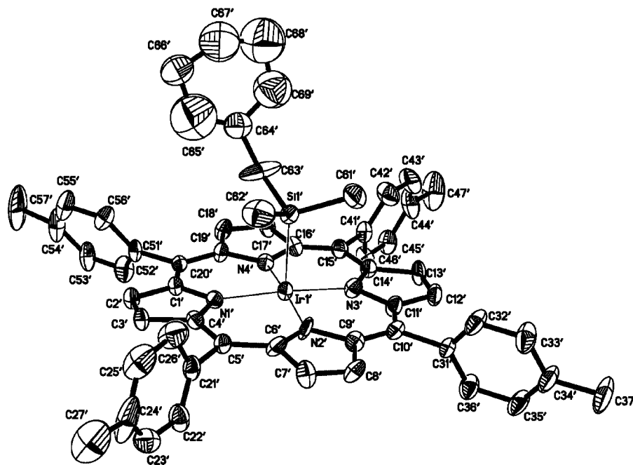
Figure 3. Molecular structure of Ir(ttp)SiBnMe 2 (30% thermal ellipsoids).
