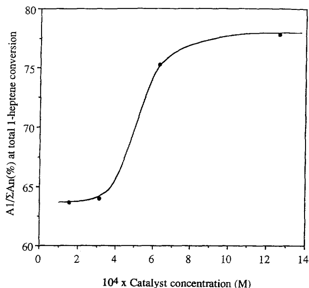
Fig. 3. Effect of catalyst concentration. Catalyst: [\text{Rh}(\mu\text{-SC}_6\text{F}_5)(\text{COD})]_2 1 . Molar ratio P/Rh = 2. An = Aldehyde ( n = 1, 2, 3 ). Temperature = 343 K; P_T = 30 bar ( \text{CO}/\text{H}_2 = 1/1 ).
