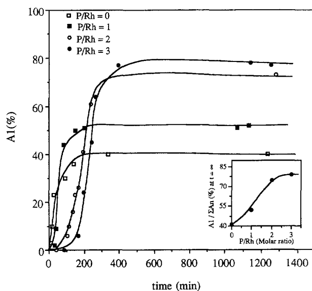
Fig. 5. Effect of P/Rh molar ratio on A1 selectivity. Catalyst: [\text{Rh}(\mu\text{-SC}_6\text{F}_5)(\text{COD})]_2 1 . Catalyst concentration = 6.29 \times 10^{-4} M. Temperature = 343 K; P_T = 30 bar ( \text{CO}/\text{H}_2 = 1/1).
