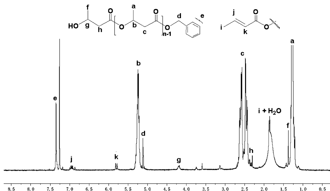
Figure 7. ^1\text{H} NMR spectrum of rac -BBL oligomer initiated by complex 5 in \text{CDCl}_3 ( [\text{rac-BBL}]_0:\mathbf{5} = 20:1 , 25^\circ\text{C} ).
