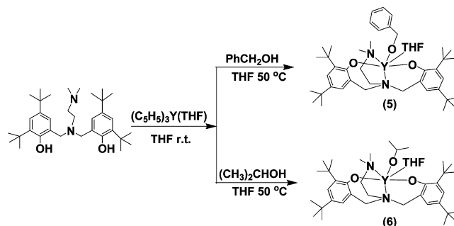
Scheme 2. Synthesis of Complexes 5 and 6
