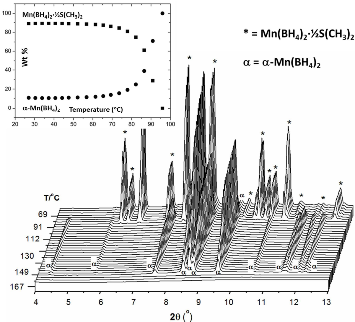
Figure 4. In situ synchrotron radiation powder X-ray diffraction measured from room temperature to 200 °C of Mn(BH 4 ) 2 ·½S(CH 3 ) 2 ( \lambda = 0.696713 \text{ \AA} , p(\text{Ar}) = 1 \text{ bar} ). Inset: Integrated intensities (wt%) of Mn(BH 4 ) 2 ·½S(CH 3 ) 2 and α-Mn(BH 4 ) 2 as a function of temperature. Filled circles: α-Mn(BH 4 ) 2 , filled squares: Mn(BH 4 ) 2 ·½S(CH 3 ) 2 .
