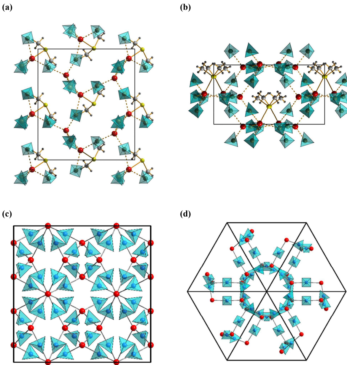
Figure 1. Crystal structure of \text{Mn}(\text{BH}_4)_2 \cdot \frac{1}{2} \text{S}(\text{CH}_3)_2 viewed along the (a) a - and (b) c -axis and the structure of \gamma\text{-Mn}(\text{BH}_4)_2 viewed along (c) the a -axis and (d) [111] . M-H bonds are omitted for clarity and Mn-B coordinations are shown instead (Mn: red, S: yellow, C: light gray, H: gray, \text{BH}_4 : blue tetrahedra).
