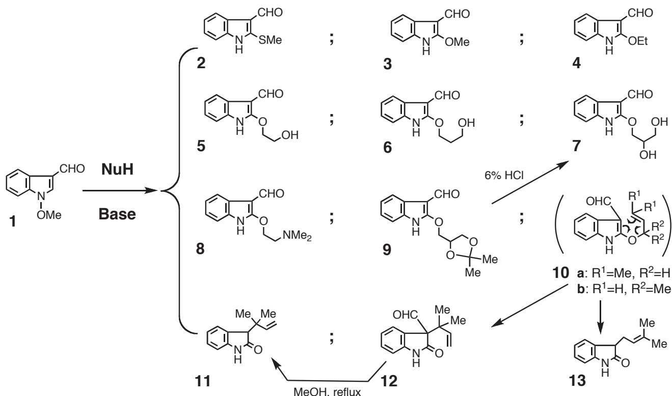
Scheme 2. Reaction of 1 with Sulfur- and Oxygen-Centered Nucleophiles
