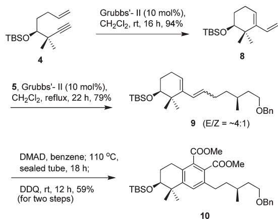
Scheme 3. Synthesis of Isofregenedadiol Skeleton through Sequential Method
