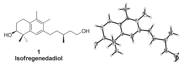
Figure 2. ORTEP diagram of the synthetic isofregenedadiol.
