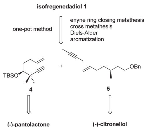
Scheme 1. Retrosynthesis
