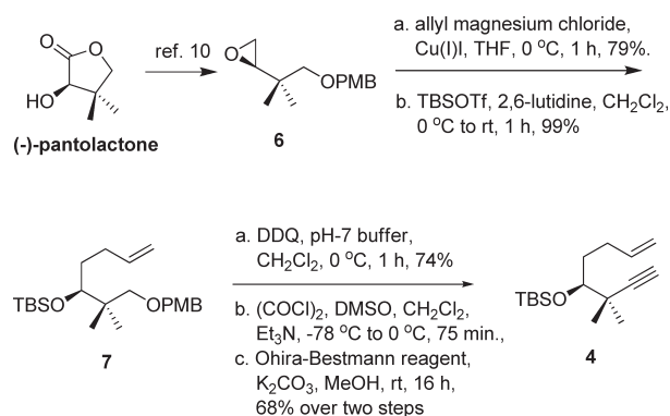
Scheme 2. Synthesis of Key Enyne Precursor 4
