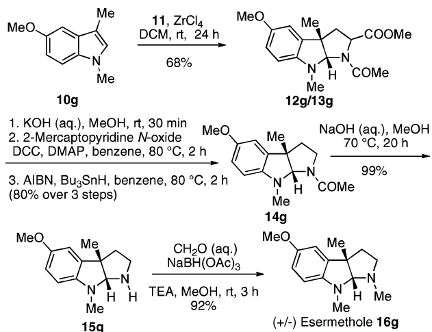
Scheme 1. Synthesis of Esermethole
