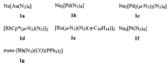
Scheme 1. Starting materials (μ-N 3 = bridging azide; Cp* = η-C 5 Me 5 ; C 10 H 14 = 4-isopropyl toluene).
