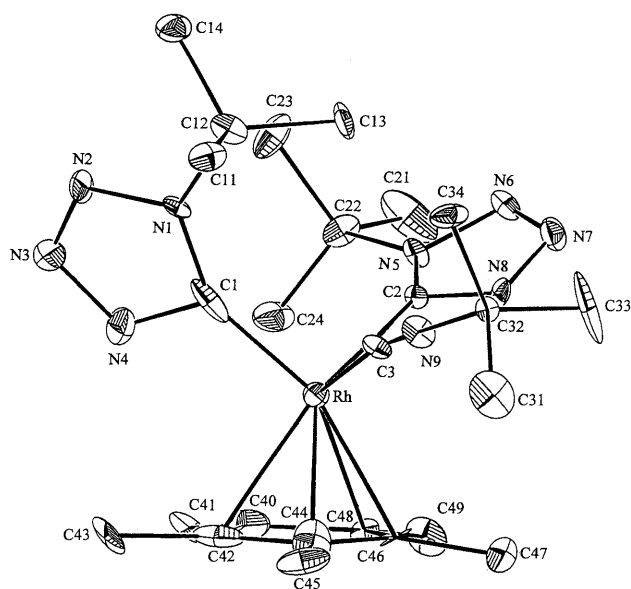
Fig. 1. ORTEP drawing of one molecule of 4a (The bonding parameters of the independent second molecule in the asymmetric unit differ only marginally.). Selected bond distances (Å) and angles (°) (averaged values over the two molecules): Rh–Cp* 2.25; Rh–C(isocyanide) 1.92(5); Rh–C(tetrazole) 2.03(5); C–N(isocyanide) 1.18(5); C–N1 1.40(5); N1–N2 1.36(6); N2–N3 1.29(6); N3–N4 1.36(6); N4–C 1.40(6) (all tetrazole); Rh–C–N(isocyanide) 170(3); N1–C–N4 104(3); C–N1–N2 110(4); N1–N2–N3 106(4); N2–N3–N4 111(4); N3–N4–C 108(4) (all tetrazole).
