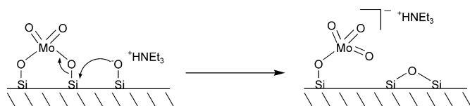
Figure 10. Possible mechanism for the formation of surface-fixed trioxomolybdenum(vi) species in the grafted material MCM-41/2/Et 3 N.
