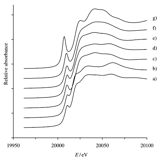
Figure 5. Mo K -edge XANES spectra of a) [\text{MoO}_2\text{Cl}_2(\text{thf})_2] ( 1 ), b) [\text{MoO}_2\text{Br}_2(\text{thf})_2] ( 2 ), c) MCM-41/1, d) MCM-41/2, e) MCM-41/1/ \text{Et}_3\text{N} , f) MCM-41/2/ \text{Et}_3\text{N} and g) \text{Na}_2\text{MoO}_4 \cdot 2\text{H}_2\text{O} .
