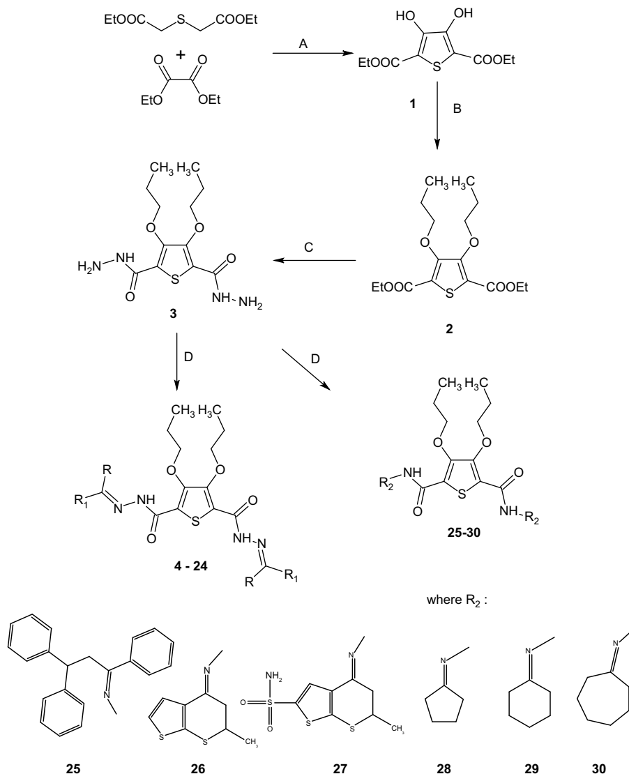
Scheme 1. Synthesis of substituted bishydrazones. A: NaOEt, H^+ ; B: CH_3CH_2CH_2Br , K_2CO_3 , DMF; C: NH_2NH_2 \cdot H_2O , EtOH; D: aldehyde/ketone, EtOH, H^+ .
