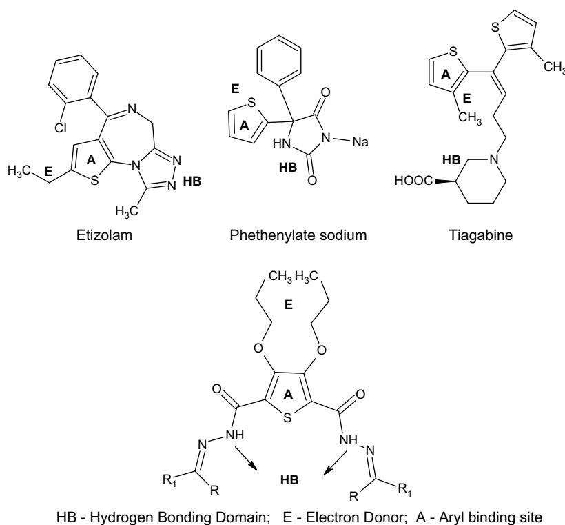
Fig. 1. Molecular design of new thiophene based antiepileptic agents by pharmacophore combination.
