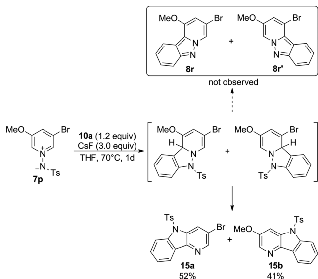
Scheme 3 Reaction with N -tosyl-3-bromo-5-methoxypyridinium imide.
