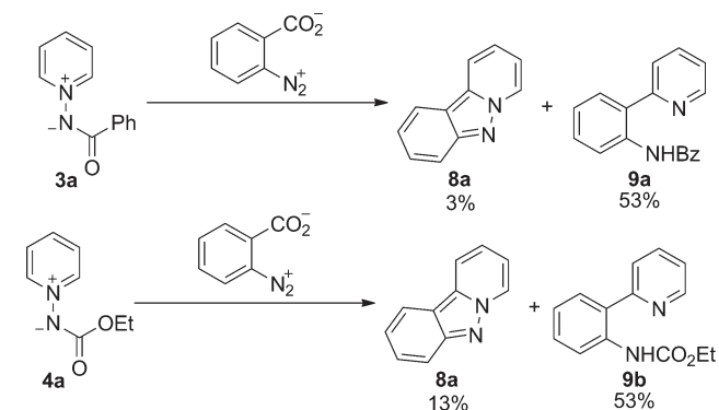
Scheme 2 Aryne [3 + 2] cycloaddition with pyridinium imide derivatives.
