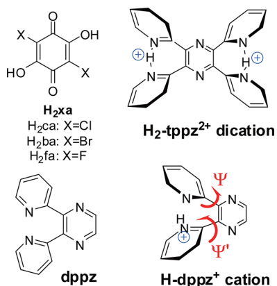
Figure 1. Chemical structures of the anilic acids ( H_2xa ) and bases. Protonated dppz and tppz can behave as proton sponges, as exemplified by H_2 -tppz 2+ , or adopt various twisted conformations by changing the dihedral angles ( \Psi and \Psi' ) between the pyrazyl and pyridyl rings.
