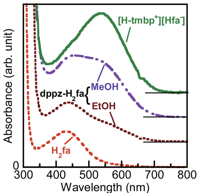
Figure 5. Electronic spectra of ethanol and methanol solutions of [dppz][H_2fa] in comparison with those of ethanol solutions of neutral H_2fa and deprotonated Hfa^- monoanion (dissolved as [H-tmbp]-[Hfa] ).
