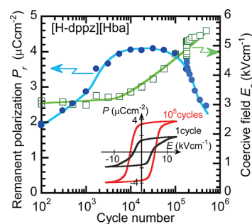
Figure 9. Fatigue behavior of the ferroelectricity in [\text{H-dppz}][\text{Hba}] crystal at room temperature. Changes in the remanent polarization P_r (solid circles) and coercive field E_c (open squares) as a function of the (total) number of continuously applied voltage pulses (rectangular waveform, f^{\text{pulse}} = 100 \text{ Hz} , E_p^{\text{pulse}} = 10 \text{ kV/cm} > E_c ). P – E hysteresis measurements with the triangular waveform voltage ( f = 1 \text{ Hz} , E_{\text{max}} = 13 \text{ kV/cm} ) were repeated with a constant interval on a logarithmic time scale. Inset: P – E hysteresis loops before and after application of the first 10^5 pulses.
