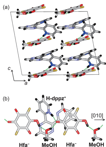
Figure 13. Crystal structures of [\text{H-dppz}][\text{Hfa}]\cdot\text{MeOH} cocrystal. (a) Molecular packing projected along the crystallographic b direction. (b) Extended supramolecular chain of alternating \text{Hfa}^- and \text{MeOH} molecules with a \text{H-dppz}^+ cation attached as a pendant.
