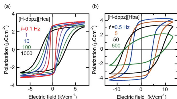
Figure 8. Electric polarization ( P )–electric field ( E ) hysteresis loops of (a) [\text{H-dppz}][\text{Hca}] and (b) [\text{H-dppz}][\text{Hba}] ( \alpha -form) crystals at room temperature. A triangular ac electric field of various frequencies was applied along the crystal c direction.
