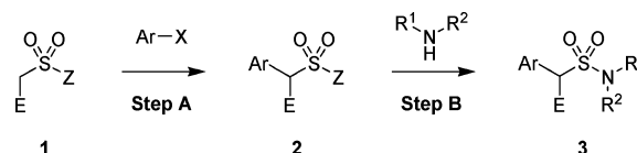
SCHEME 1. Strategy for Preparing Benzylic Sulfonamides
