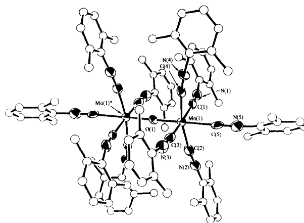
Fig. 1. Perspective drawing of the complex cation of 1a , [\text{Mo}_2(\mu\text{-O})(\text{XylNC})_{10}]^{2+} .
