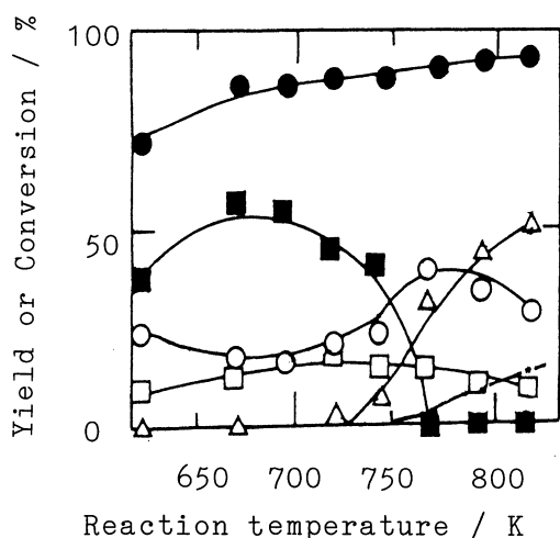
Fig. 1. Effect of reaction temperature on the conversion of methanol (●) and yield of MMA (○), DMA (□), TMA (■), \text{CH}_4 (△) and \text{N}_2 (•). Catalyst: \text{NH}_4\text{PW} . W/F=0.3 \text{ g-cat}^{-1}\text{min cm}^{-3} .
