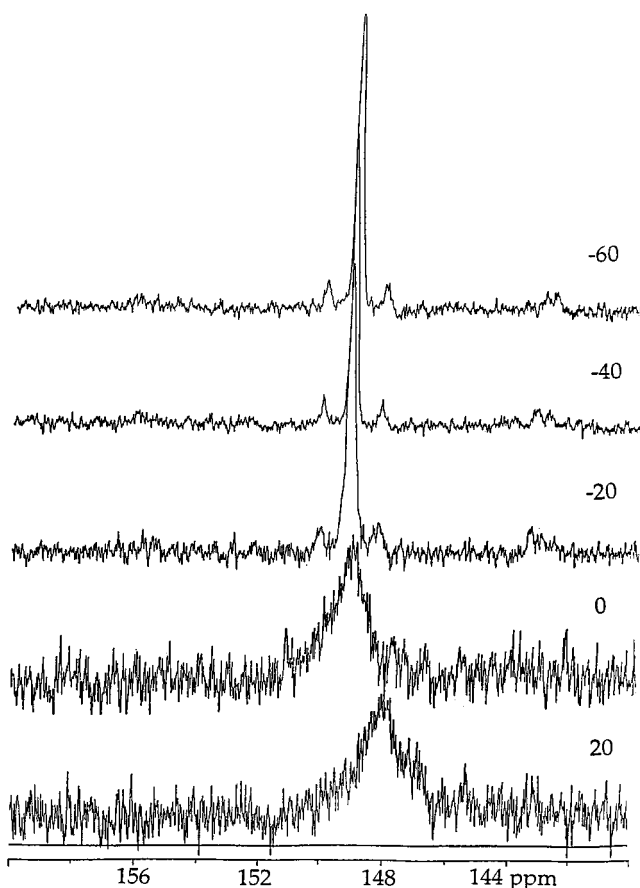
Figure 3. 50 MHz dynamic 13 C NMR spectra of 1 obtained from a solution of the complex in THF- d 6 . Numbers indicate temperatures (°C) at which spectra were obtained.
