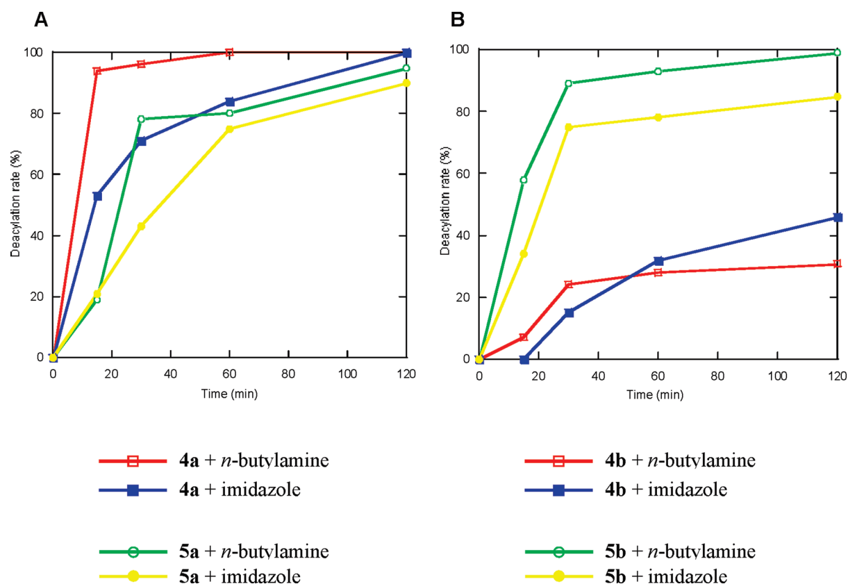
Figure 5. (A) Kinetic analysis of the deacylation of mono-2'(3')-O-alanyl-AMP ( 4a ) and mono-2'(3')-O-alanyl-UMP ( 5a ) in the presence of 2 equiv of n -butylamine (red and green, respectively) and imidazole (blue and yellow, respectively). (B) Kinetic analysis of the deacylation of bis-2',3'-O-alanyl-AMP ( 4b ) and bis-2',3'-O-alanyl-UMP ( 5b ) in the presence of 2 equiv of n -butylamine (red and green, respectively) and imidazole (blue and yellow, respectively). The percent formation of AMP and UMP after treatment is shown over a period of 120 min as analyzed by reversed-phase HPLC (250 × 4.6 mm, 5 μm column). The column was washed with 0% → 63% CH 3 CN in 50 mM NH 4 OAc, pH 4.5, over a period of 35 min at a flow rate of 1 mL/min (monitoring at 260 nm). Aliquots were analyzed after 15, 30, 60, and 120 min.
