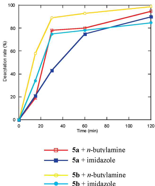
Figure 6. Kinetic analysis of the deacylation of mono-2'-(3')-O-alanyl-UMP ( 5a ) and bis-2',3'-O-alanyl-UMP ( 5b ) in the presence of 2 equiv of n -butylamine (red and yellow, respectively) and imidazole (dark blue and light blue, respectively). The percent formation of UMP after treatment is shown over a period of 120 min as analyzed by reversed-phase HPLC (250 × 4.6 mm, 5 μm column). The column was washed with 0% → 63% CH 3 CN in 50 mM NH 4 OAc, pH 4.5, over a period of 35 min at a flow rate of 1 mL/min (monitoring at 260 nm). Aliquots were analyzed after 15, 30, 60, and 120 min.
