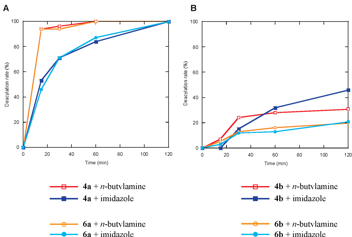
Figure 4. (A) Kinetic analysis of the deacylation of mono-2'(3')-O-alanyl-AMP ( 4a ) and mono-2'(3')-O-alanyl-pdCpA ( 6a ) in the presence of 2 equiv of n -butylamine (red and orange, respectively) and imidazole (dark blue and light blue, respectively). (B) Kinetic analysis of the deacylation of bis-2',3'-O-alanyl-AMP ( 4b ) and bis-2',3'-O-alanyl-pdCpA ( 6b ) in the presence of 2 equiv of n -butylamine (red and orange, respectively) and imidazole (dark blue and light blue, respectively). The percent formation of AMP and pdCpA after treatment is shown over a period of 120 min as analyzed by reversed-phase HPLC (250 × 4.6 mm, 5 μm column). The column was washed with 0% → 63% CH 3 CN in 50 mM NH 4 OAc, pH 4.5, over a period of 35 min at a flow rate of 1 mL/min (monitoring at 260 nm). Aliquots were analyzed after 15, 30, 60, and 120 min.
