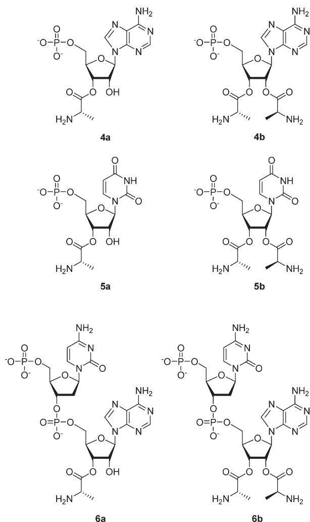
Figure 3. Compounds synthesized and studied for their reactivity toward nucleophiles. Mono-2'-(3')-O-alanyl-AMP ( 4a ), bis-2',3'-O-alanyl-AMP ( 4b ), mono-2'-(3')-O-alanyl-UMP ( 5a ), bis-2',3'-O-alanyl-UMP ( 5b ), mono-2'-(3')-O-alanyl-pdCpA ( 6a ), and bis-2',3'-O-alanyl-pdCpA ( 6b ).
