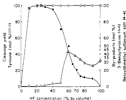
Figure 2. Plot for the products obtained from the deprotection of Tyr(Bzl) in different concentrations of HF in dimethyl sulfide at 0 °C for 1 h: (□) cleavage yield; (●) benzyldimethylsulfonium ion, (Δ) 3-benzyltyrosine.
