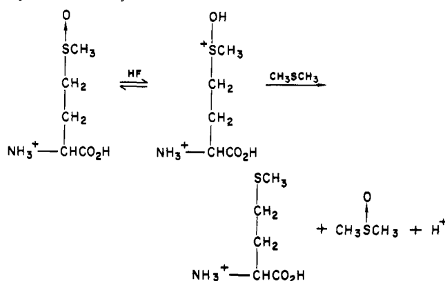
Scheme IV. Reduction of Methionine Sulfoxide to Methionine by HF in Dimethyl Sulfide
