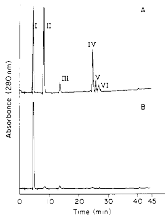
Figure 4. HPLC analysis of HF-thiol deprotection of N f -formyltryptophan at 0 °C: (A) high HF procedure, HF- p -thiocresol- p -cresol (90:5:5, v/v), and (B) low HF procedure, HF-DMS- p -thiocresol- p -cresol (25:65:5:5, v/v, 2 h), and then high HF procedure (same as A). I, Trp; II, Trp(For); III, p -cresol; IV-VI, Trp- p -thiocresol side products.
