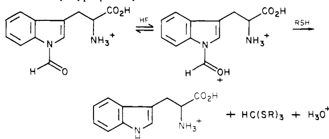
Scheme V. Proposed Mechanism for the Deprotection of N i -Formyltryptophan by Thiol in HF
