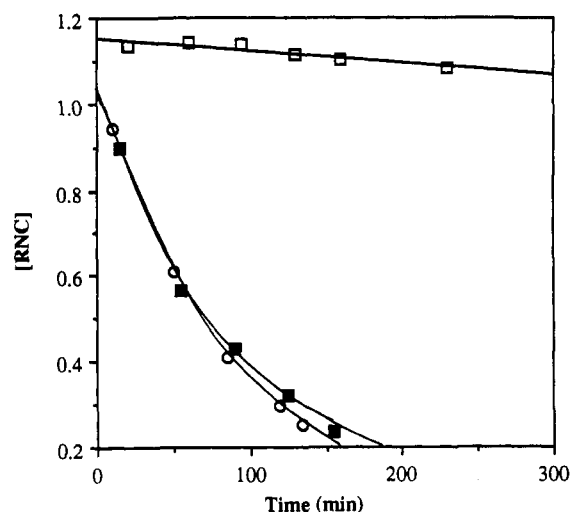
Figure 7. Rates of disappearance of ( \pm )-II versus time under oxygen for different catalysts: (allyl)Ni(II)Br + 3PPh 3 (black squares), (PPh 3 ) 3 -Ni(I)Br (white circles), and (PPh 3 ) 2 Ni(II)Br 2 + PPh 3 (white squares). All have identical initial concentrations of nickel and monomer.
