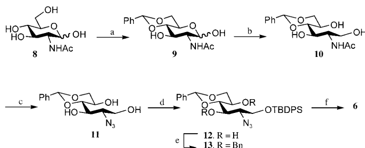
Scheme 3. a) PhCHO, ZnCl 2 ; b) NaBH 4 , MeOH; c) Ba(OH) 2 ·8H 2 O, MeOH, H 2 O, 90 °C; then Tf 2 O, NaN 3 , CuSO 4 ; d) TBDPSCl, imidazole, DMF; e) BnBr, NaH, DMF; f) 1 M BH 3 in THF, 1 M Bu 2 BOTf in CH 2 Cl 2 . Tf = trifluoromethanesulfonyl.
