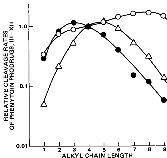
Figure 4 —Ratio of the rate constants for the cleavage of compounds III–VI, VII–XII to phenytoin in human (●) and rat (○) plasma and rat intestinal homogenates (△) at 37° to the 3-pentanoyloxymethyl derivative, VI, against alkyl chain length of the acyl function.
