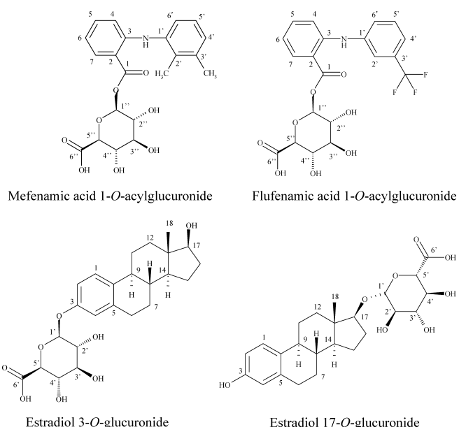
Fig. 2. Chemical Structures of Four Glucuronides Prepared in This Study
