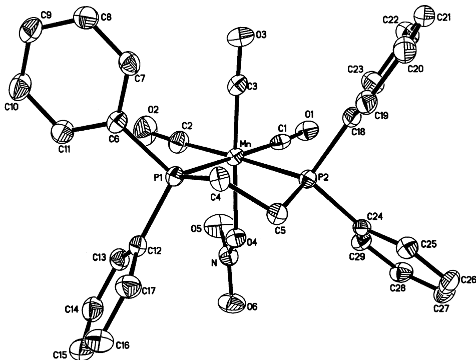
Fig. 1. ORTEP diagram of fac -Mn(CO) 3 (dppe)NO 3 ( 2 ), indicating labeling scheme and 50% thermal ellipsoids.
