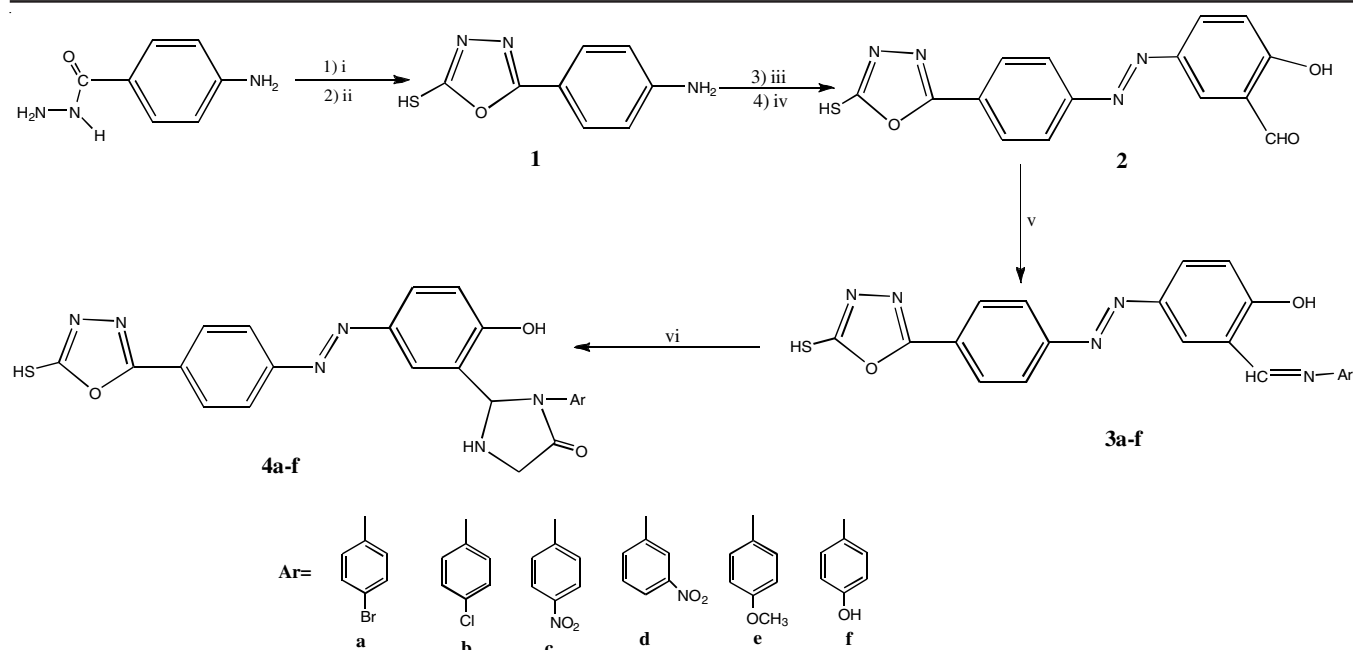
Scheme-I: Synthesis of imidazolidines, Reagents and conditions (i) \text{CS}_2 , KOH, EtOH, 70 °C, 24 h; (ii) conc. HCl; (iii) \text{NaNO}_2 , HCl, 0-5 °C; (iv) 2-hydroxybenzaldehyde, NaOH 10 %, 5 °C; (v) Ar- \text{NH}_2 , EtOH, MW (300W), 25 min; (vi) glycine, tetrahydrofuran, MW (450-500 W), 45 min
