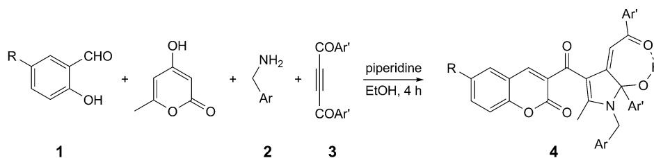
Scheme 1. Synthesis of 3-[(4,5-Dihydro-1H-pyrrol-3-yl)carbonyl]-2H-chromen-2-ones. For R, Ar, and Ar', see the Table .
