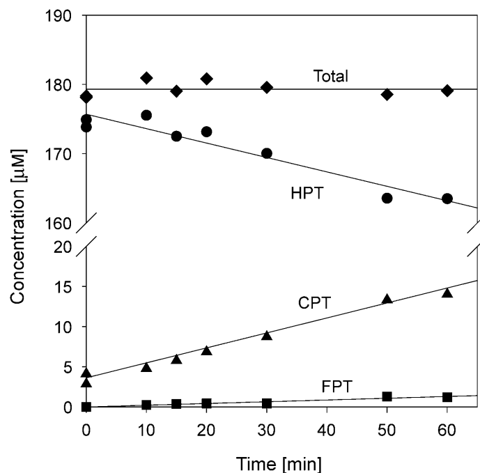
Fig. 4. Evolution of the HPLC-based concentrations of HTP ( 1a ), FTP ( 5 ), and CPT ( 6 ). The initial concentration of 1a was 180 µM. The aq. solutions (pH 5.5) were irradiated in the absence of O 2 , and aerated in the dark immediately after irradiation. The mathematical sum (◆) of the different experimental concentrations is also shown.
