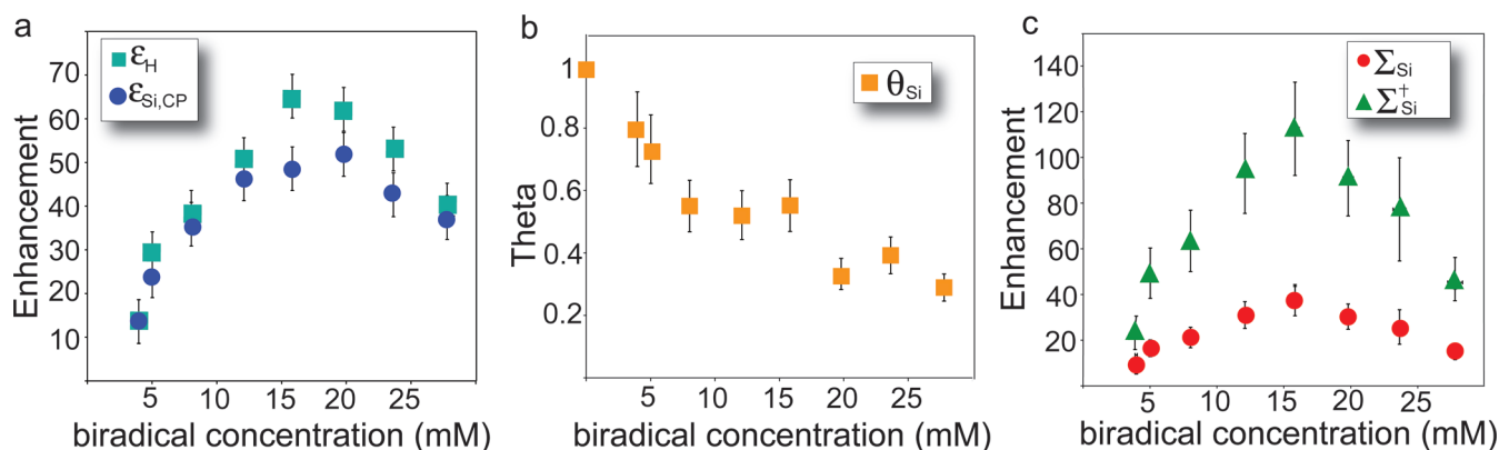
Figure 2. (a) Proton DNP ( \epsilon_H ) and silicon DNP enhancement ( \epsilon_{Si,CP} ). (b) The ^{29}\text{Si} quenching factor ( \theta_{Si} ) shown as a function of bCTbK concentration in 1,1,2,2-tetrachloroethane. (c) Overall ( \Sigma_{Si,CP} and \Sigma_{Si}^+ ) sensitivity enhancements. Note that \epsilon_H quantifies the enhancement of the solvent and \epsilon_{Si,CP} quantifies that of the surface. Experimental details and definition of the enhancement factors are given in the Supporting Information.
