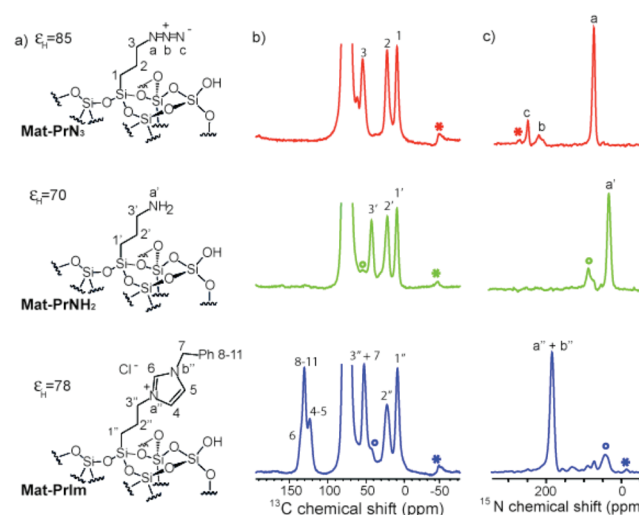
Figure 4. (a) Structure, (b) ^1\text{H} – ^{13}\text{C} CP spectra, and (c) ^1\text{H} – ^{15}\text{N} spectra of compounds Mat-PrN 3 , Mat-PrNH 2 , and Mat-PrIm . The most probable assignments based on the observed chemical shift resulting from this spectrum are shown. The asterisks indicate spinning sidebands, and the open circles note the presence of byproducts or incomplete conversion from the previous synthetic steps. The proton enhancements with a sample spinning frequency of 12 kHz are also reported. Experimental details are described in the text and in the Supporting Information.
