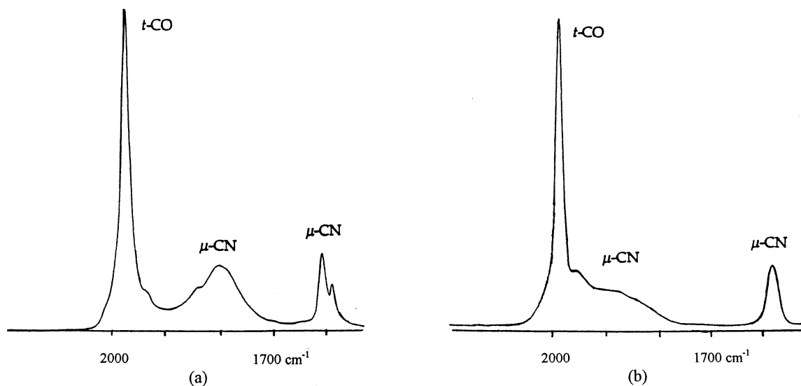
Fig. 2. The inheired spectrum of trans -[Fe 2 (η-C 5 H 5 ) 2 (CO) 2 (μ-CNMe)(μ-CNMe 2 )] [SO 3 CF 3 ], [25][SO 3 CF 3 ], in (a) the solid state (KBr) and (b) CH 2 Cl 2 solution.
