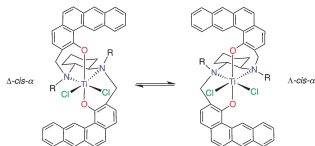
Figure 1. Exchange between diastereomeric \Delta and \Lambda helical \alpha - cis -coordinated ligands.
