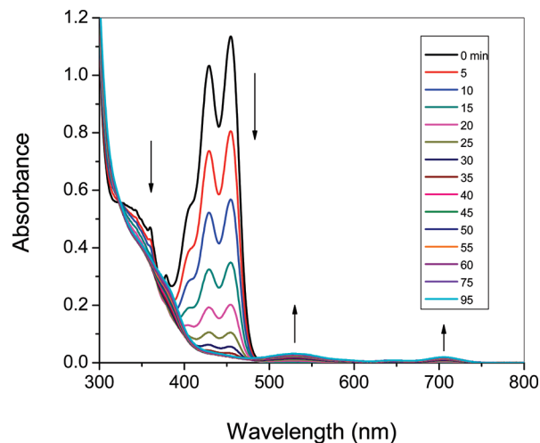
Figure 4. UV–vis absorption spectra of an air-saturated \text{CDCl}_3 solution of 1 at different irradiation time. Conditions: light intensity = 80 W, wavelength = 300–500 nm. The arrows indicate directions of absorbance changes.
