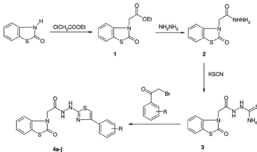
Scheme 1. The synthetic protocol of the title compounds ( 4a–j ).
