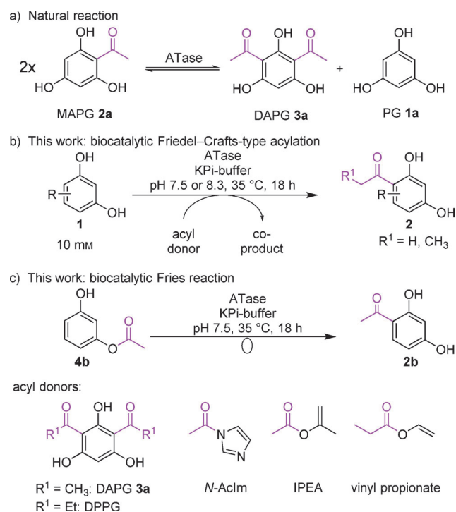
Scheme 1. Reactions catalyzed by acyltransferases from Pseudomonas fluorescens . a) Natural reaction: disproportionation of monoacetylphloroglucinol [MAPG ( 2a )] into 2,4-diacetylphloroglucinol [DAPG ( 3a )] and phloroglucinol [PG ( 1a )]. Non-natural reactions involve: b) The Friedel–Crafts bioacylation of resorcinols ( 1 ) into the corresponding aryl ketones 2 by using various acyl donors. c) Enzymatic Fries-like rearrangement reaction of phenolic esters ( 4 ) to give aryl ketones ( 2 ) as exemplified by the rearrangement of 4b into 2b .
