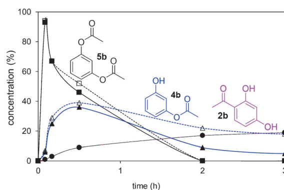
Figure 1. Time progression curves for the overall PpATaseCH -catalyzed acetylation of 1b (10 mM) with N -AcIm (250 mM). Reaction was monitored in the presence (solid lines, filled symbols) and absence (dashed lines, open symbols) of the enzyme. The relative amounts of the product 2b (magenta, ●), monoester 4b (blue, ▲), and diester 5b (dark blue, ■) were determined by HPLC. Symbols represent the mean of two ( n = 2) experiments.
