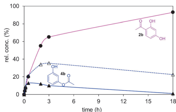
Figure 3. Time course of the PpATaseCH Friedel–Crafts bioacetylation of 1b (10 mM) with IPEA (100 mM) in the presence of imidazole (100 mM). Reaction was monitored in the presence (solid lines, filled symbols) and absence (dashed lines, open symbols) of enzyme. The relative amounts of product 2b (magenta, ●) and monoester 4b (blue, ▲) were determined by HPLC. The missing amount corresponds to the concentration of 1b .
