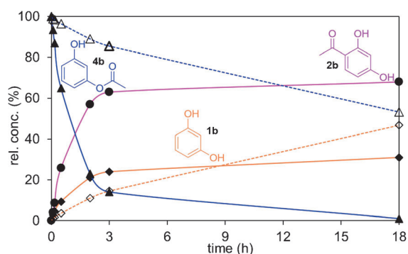
Figure 2. Time course of the PpATaseCH -catalyzed bio-Fries reaction of 4b (10 mM) to give 2b , and spontaneous hydrolysis of 4b leading to 1b . Reaction was monitored in the presence (solid lines, filled symbols) and absence (dashed lines, open symbols) of enzyme. The relative amounts of 2b (magenta, ●), monoester 4b (blue, ▲), and 1b (orange, ◆) were determined by HPLC. Symbols represent the mean of two ( n=2 ) experiments.
