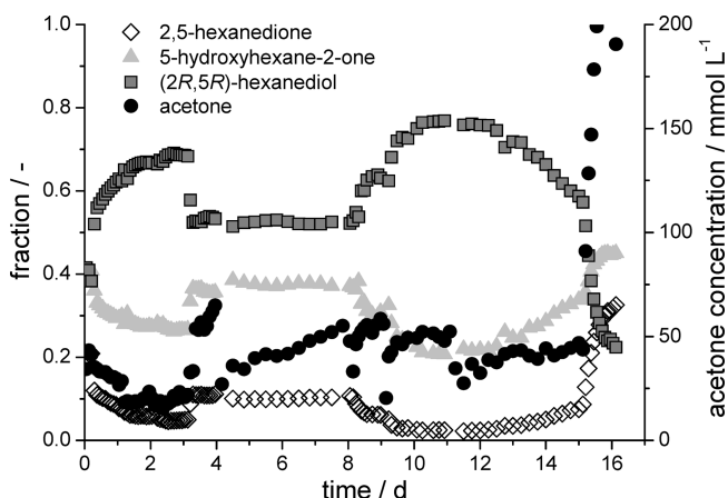
Figure 4. Fraction of 2,5-hexanedione, 5-hydroxyhexane-2-one, (2 R ,5 R )-hexanediol, and acetone concentration during a continuously operated biotransformation process with in situ acetone removal by pervaporation. Process conditions: see Table 2.
