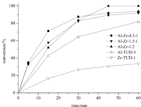
Figure 11. Intramolecular Prins cyclisation of (±)-citronellal (4 mmol) in toluene (5 g) at 80 °C using different TUD-1 catalysts (50 mg) with Si/M ratio of approximately 25: Al-Zr-4.3:1, Al-Zr-1.5:1, Al-Zr-1:2, Al-TUD-1 and Zr-TUD-1.
