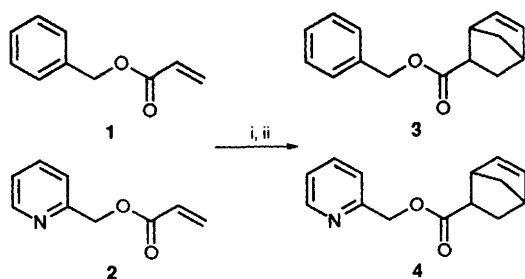
Scheme 1 Reagents and conditions: i, cyclopentadiene (5 equiv.), catalyst, solvent (see Tables), -10^\circ\text{C} , 16–18 h; ii, aq. EDTA workup
