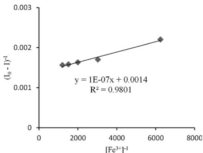
Fig. 10 Variation of (I_0 - I)^{-1} of emission as a function of [Fe^{3+}]^{-1} for SBA-F
