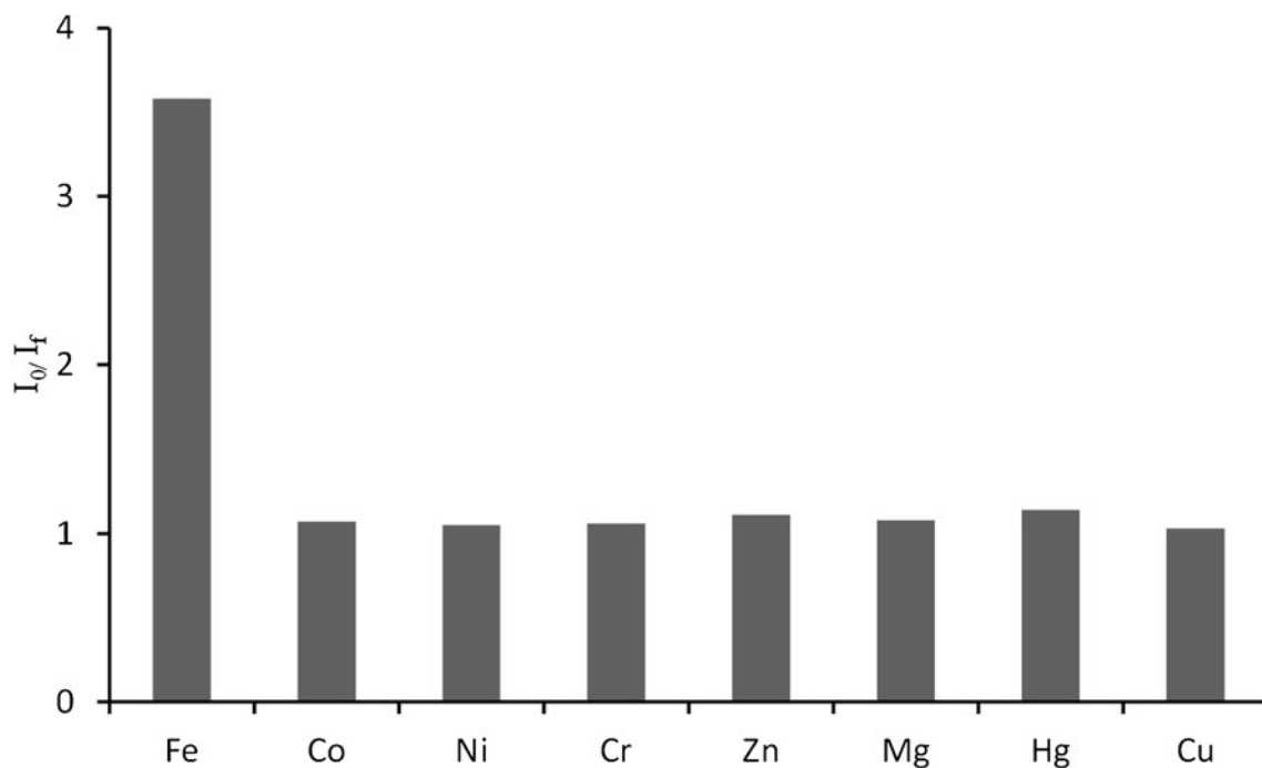
Fig. 8 Bar graphs of the fluorescence emission intensity for Fe^{3+} , Co^{2+} , Ni^{2+} , Cr^{3+} , Zn^{2+} , Mg^{2+} , Hg^{2+} and Cu^{2+} metal ions showing the metal ions selectivity profile of SBA-F (200 \mu g/2.0 mL) with a concentration of
